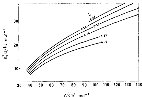
Figure 3. Vaporization energy \Delta_v^0 U for straight-chain hydrocarbons (after Blanks and Prausnitz 54 and used with permission of the American Chemical Society).
